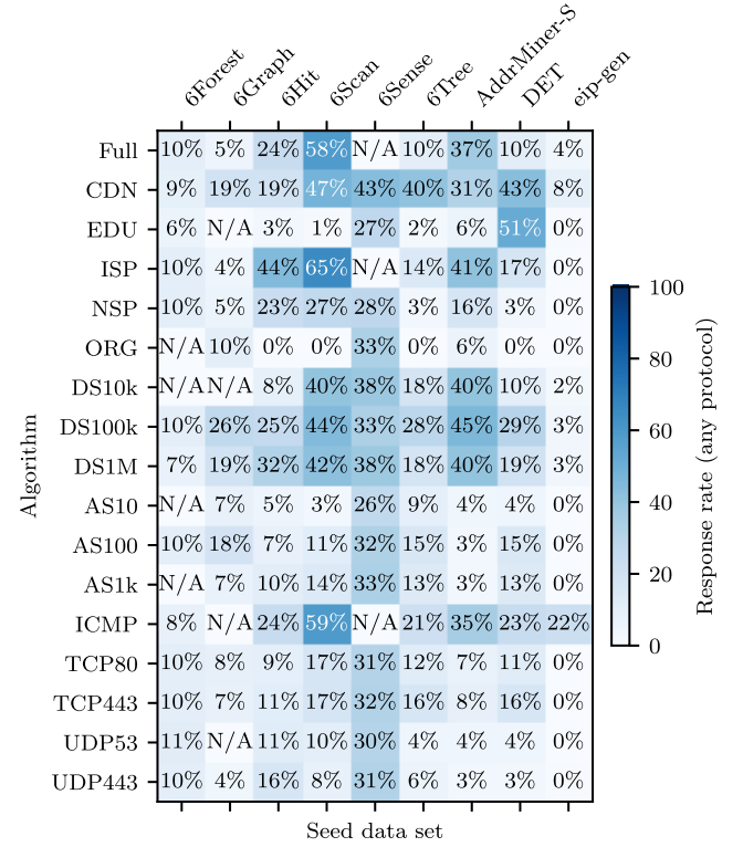
Fig. 10. Relative hit rates per algorithm and input seed set from our 2025 evaluation.
