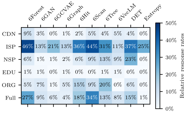
Fig. 5. Relative response rate for every candidate set generated by the TGAs with different categorized input sets as well as the full hitlist as input in 2023.
