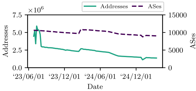
Fig. 9. Responsiveness of addresses added to the IPv6 Hitlist service over time. In total 9.1 M new addresses were added on June 27, 2023.
