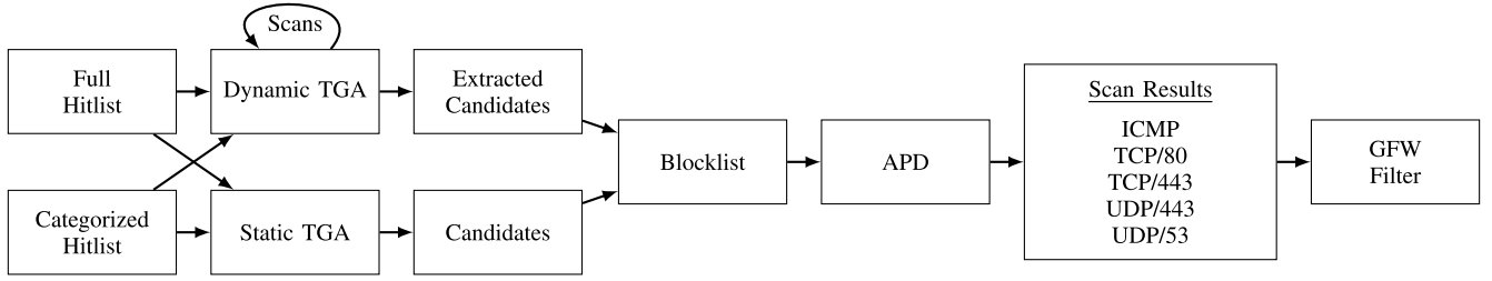
Fig. 1. Pipeline to analyze TGAs (see Table I) and their performance within different IP address categories.
