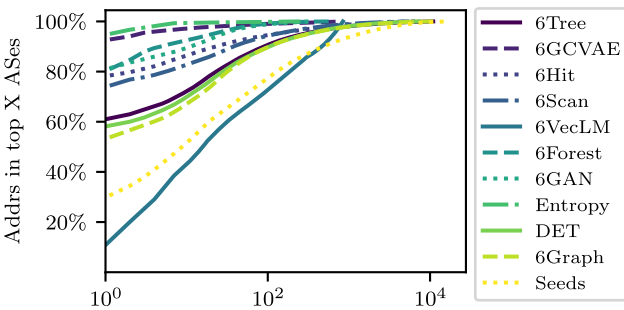
Fig. 7. Cumulative AS distribution of the responsive candidate sets generated by the algorithms using the full hitlist as input in 2023. Note the logarithmic x-axis.
