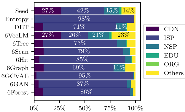
Fig. 6. Category distribution of responsive addresses from each Target Generation Algorithm applied on the full set of responsive addresses from the IPv6 Hitlist in 2023.
