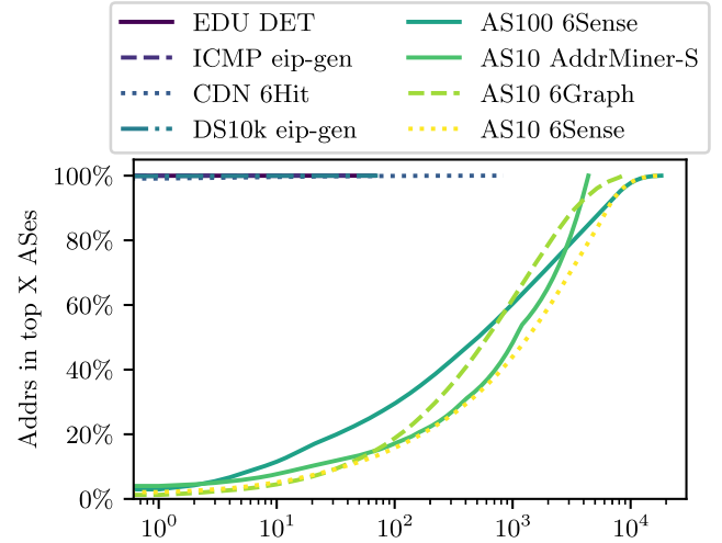
Fig. 12. AS distribution of responsive candidates with highest and lowest entropy from our 2025 evaluation. The entropy is calculated as Shannon entropy over the distribution of ASes per set.
