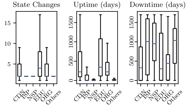
Fig. 4. Stability of responsive IPv6 addresses of the IPv6 Hitlist per category. Data from scans is used from July 2018 to March 2023, while addresses newly discovered from November 2022 onwards are excluded to reduce the impact of newer scans.
