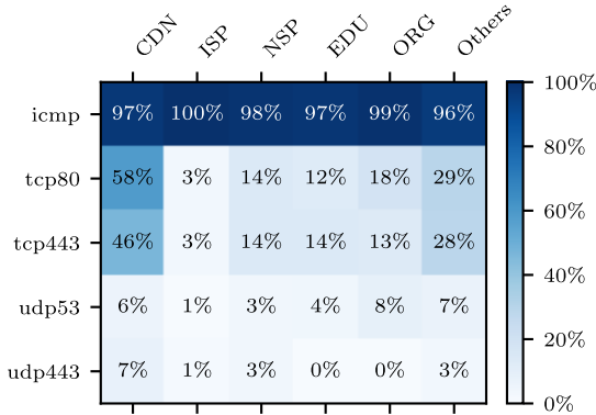
Fig. 3. Responses to the different protocols per category within the IPv6 Hitlist on March 3, 2023.
