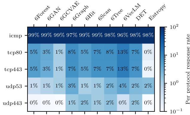
Fig. 8. Response rates to the different protocols per algorithm generated on full hitlist input in 2023. Note the color map log scale.
