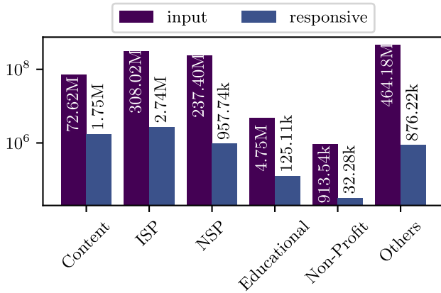
Fig. 2. Prevalence of different categories in the IPv6 Hitlist on March 3, 2023. Note the logarithmic y-axis.
